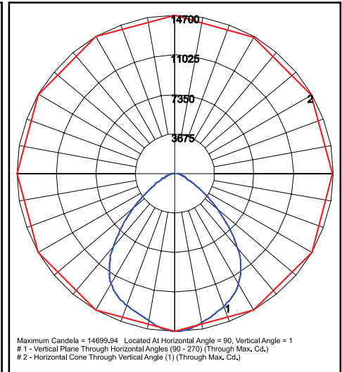
FXBLD8QM1X200U4K Grid in feet, Mounting Height = 25 ft.
