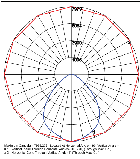
FXBLD4QM1X100U4K Grid in feet, Mounting Height = 25 ft.
