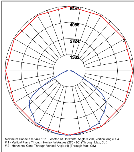
FXBLD4QW1X100U4K Grid in feet, Mounting Height = 25 ft.
