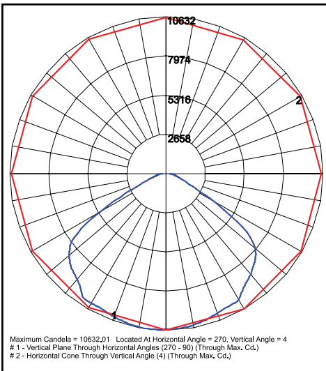
FXBLD8QW1X200U4K Grid in feet, Mounting Height = 25 ft.
