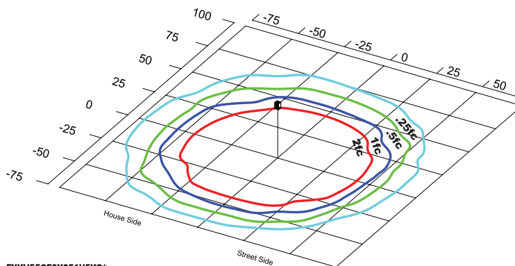
FXKH55QF2X256U5KC* Type V Grid in MH MH=25 Feet
