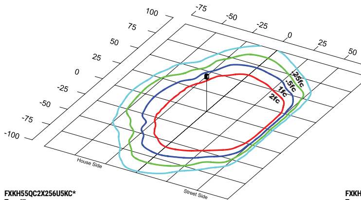
FXKH55QC2X256U5KC* Type III Grid in MH MH=25 Feet
