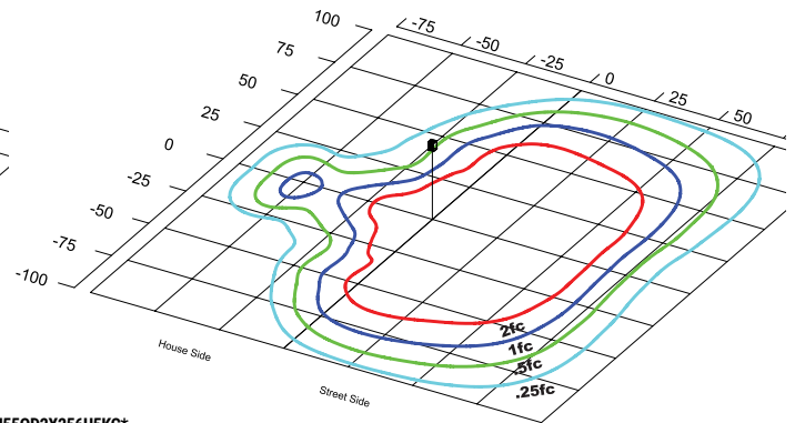
FXKH55QD2X256U5KC* Type IV Grid in MH MH=25 Feet
